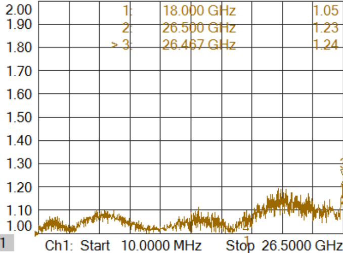
Tr 1 S11 SWR 0.100U/ 1.00U
