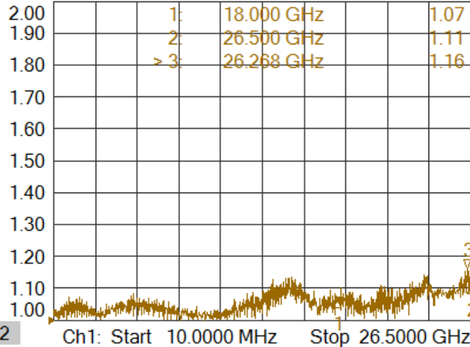
Tr 3 S22 SWR 0.100U/ 1.00U
