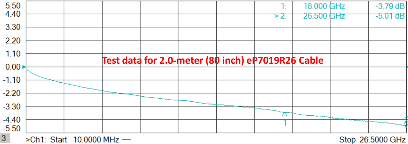
Tr 2 S21 LogM 1.100dB/ 0.00dB
